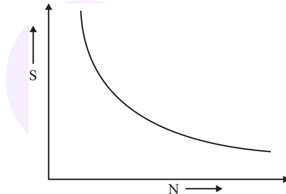
Figure: A schematic plot of reversed stress (S) against number of cycles to fail (N) for non-metals, showing the absence of knee in the plot.
