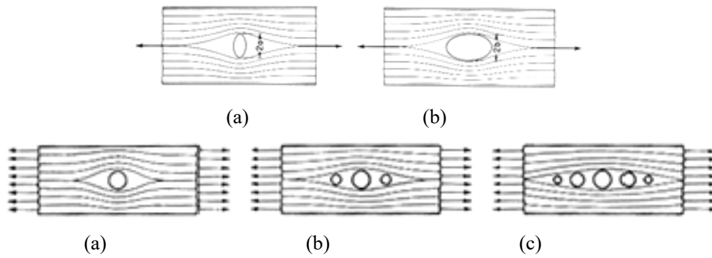
Figure: Reduction of stress concentration in tension
